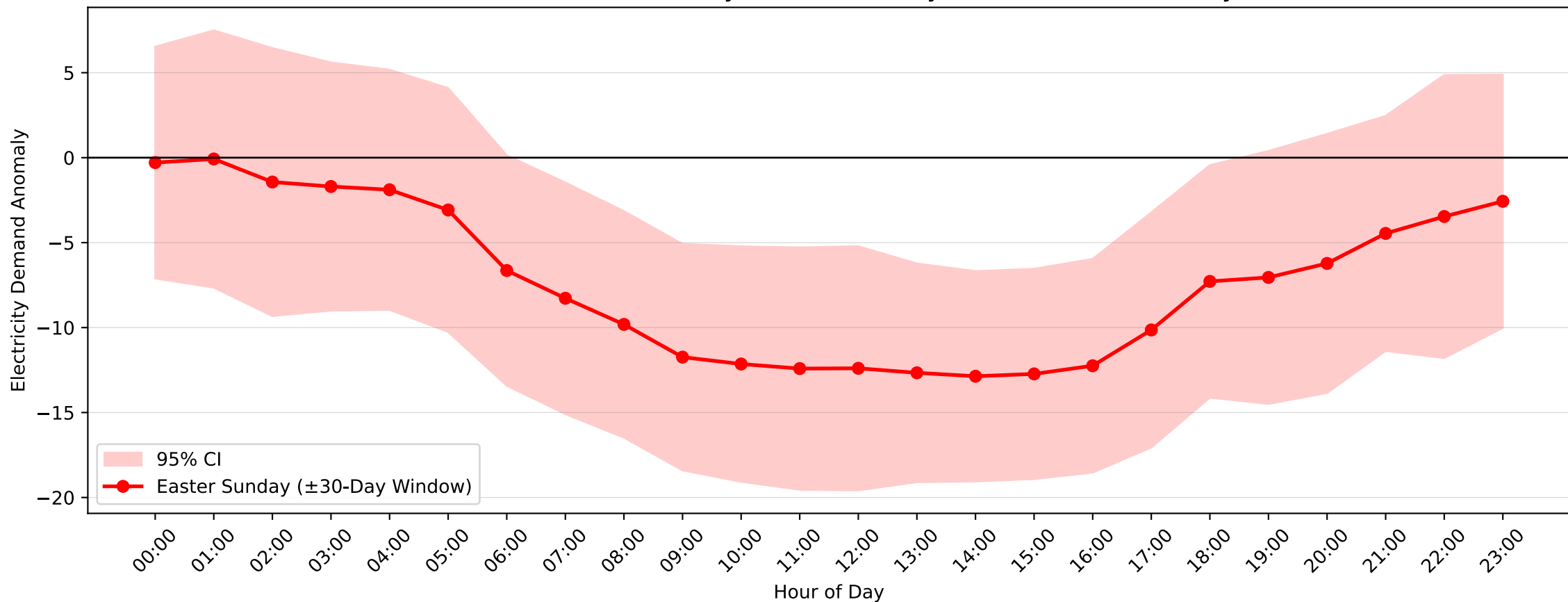
Greenacre Park Demand Anomaly: Easter Sunday (2014-2015, \pm 30 -Day Window)
