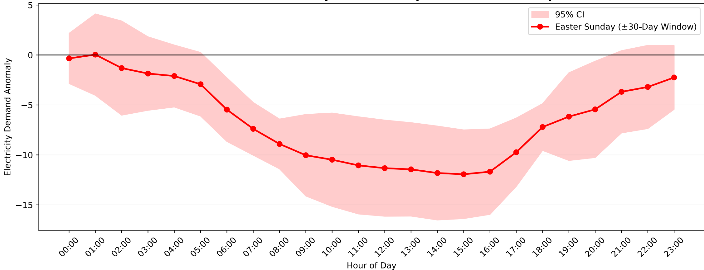
Greenacre Park Demand Anomaly: Easter Sunday (2015-2016, \pm 30 -Day Window)
