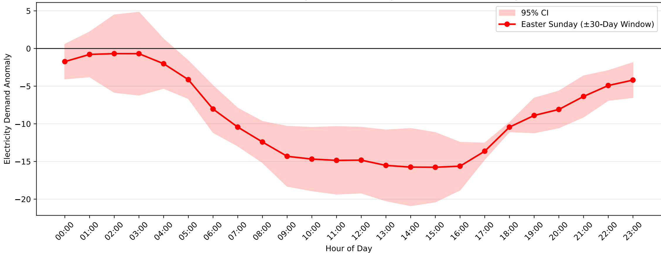
Greenacre Park Demand Anomaly: Easter Sunday (2013–2014, \pm 30 -Day Window)
