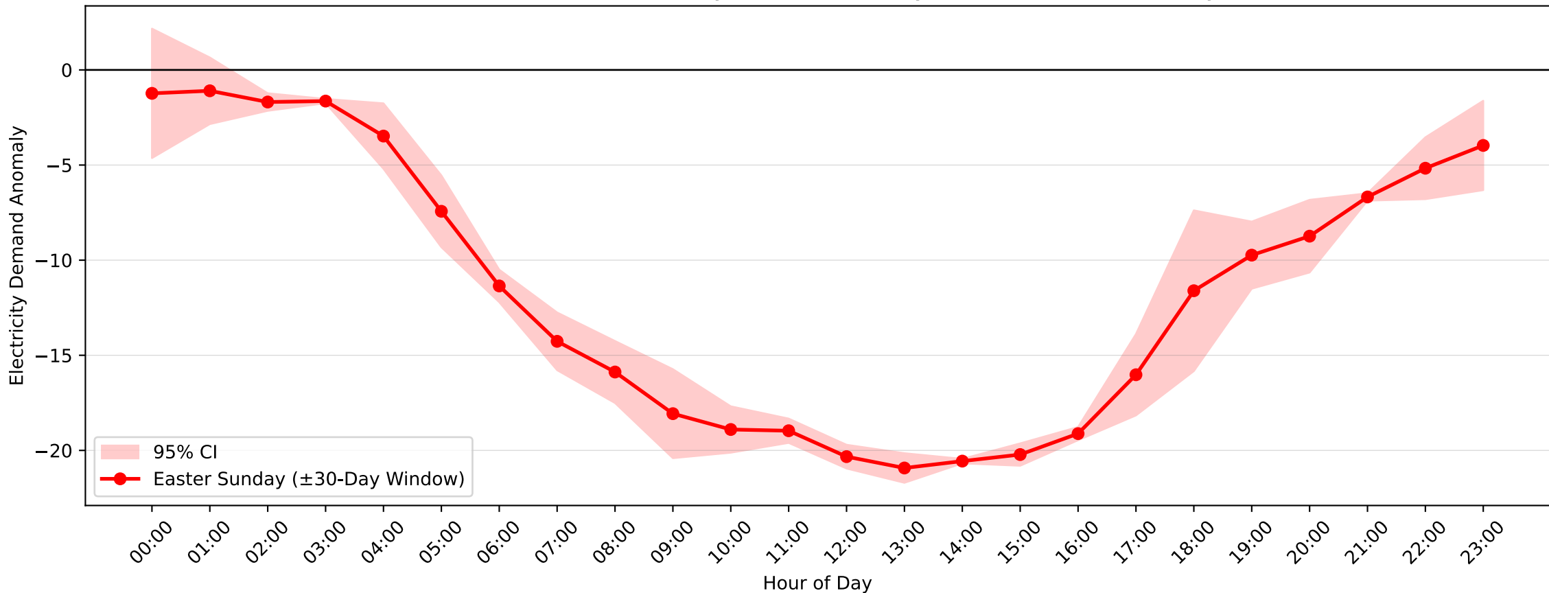
Greenacre Park Demand Anomaly: Easter Sunday (2007-2008, \pm 30 -Day Window)
