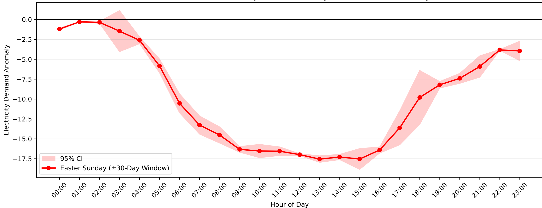
Greenacre Park Demand Anomaly: Easter Sunday (2008-2009, \pm 30 -Day Window)
