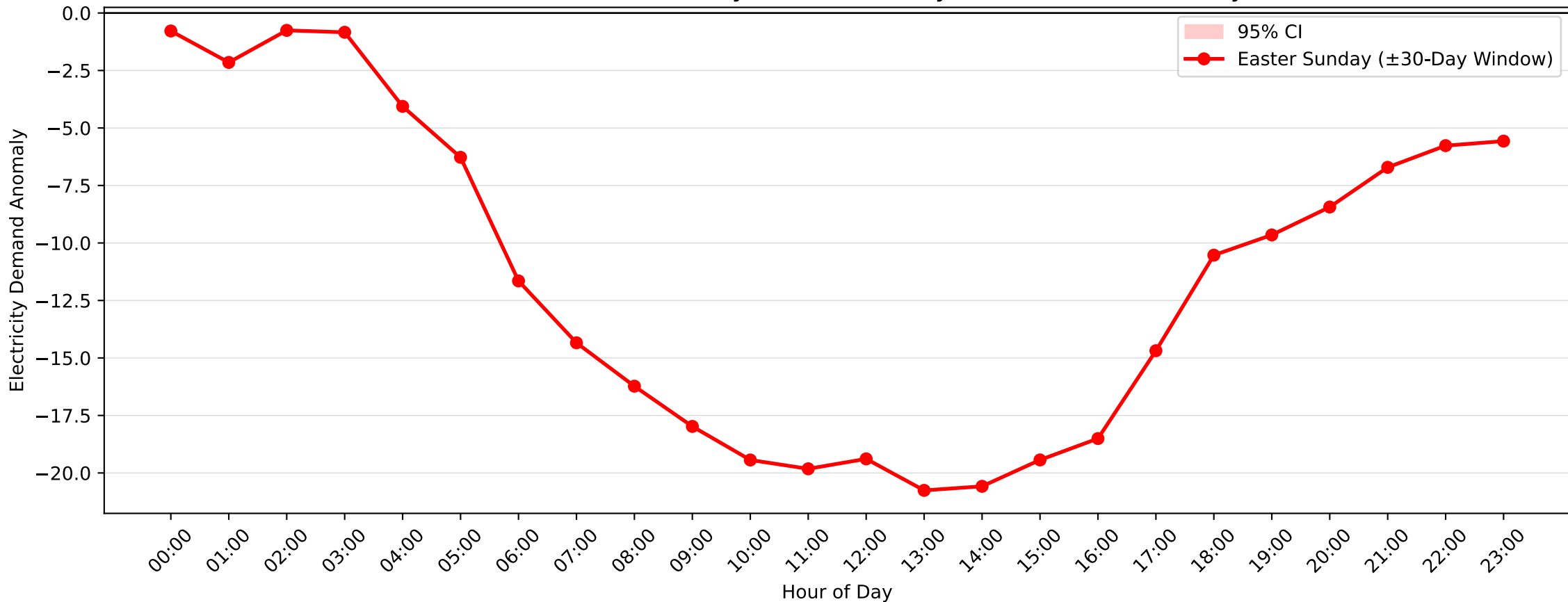
Greenacre Park Demand Anomaly: Easter Sunday (2005-2006, \pm 30 -Day Window)
