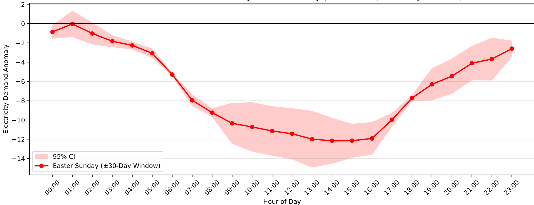
Greenacre Park Demand Anomaly: Easter Sunday (2016–2017, \pm 30 -Day Window)
