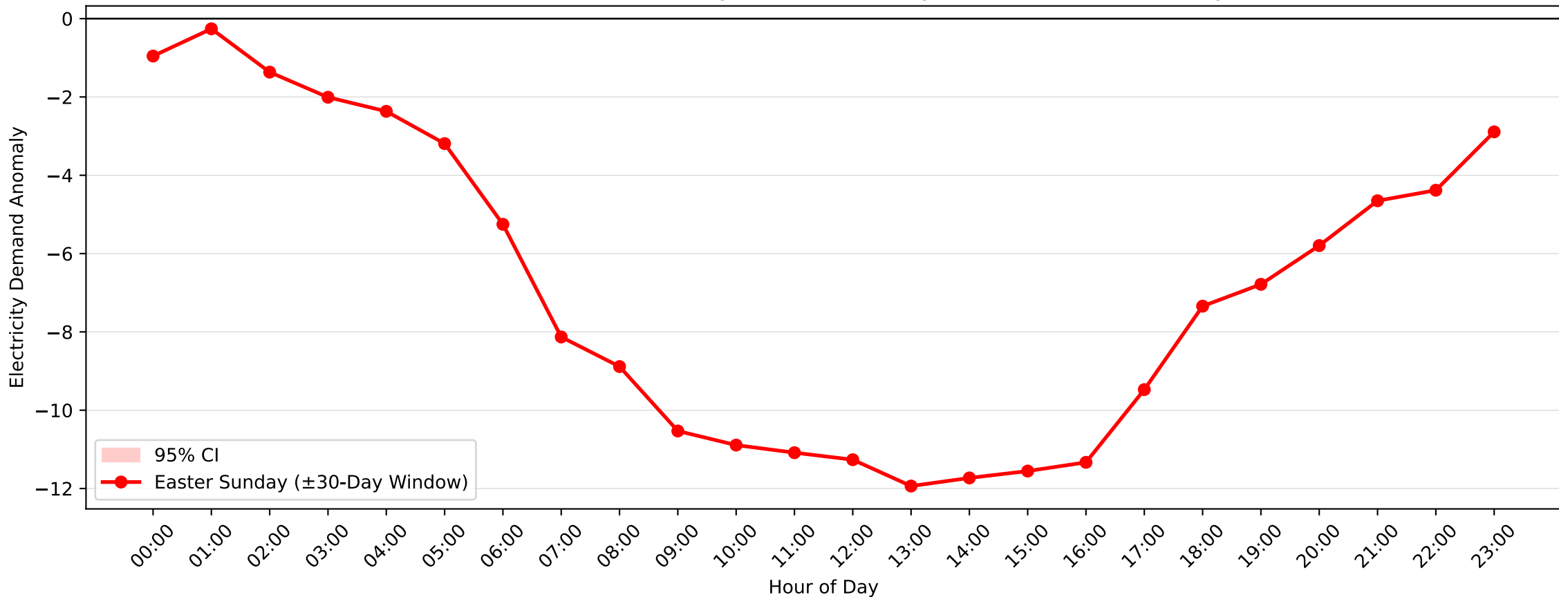
Greenacre Park Demand Anomaly: Easter Sunday (2017-2018, \pm 30 -Day Window)
