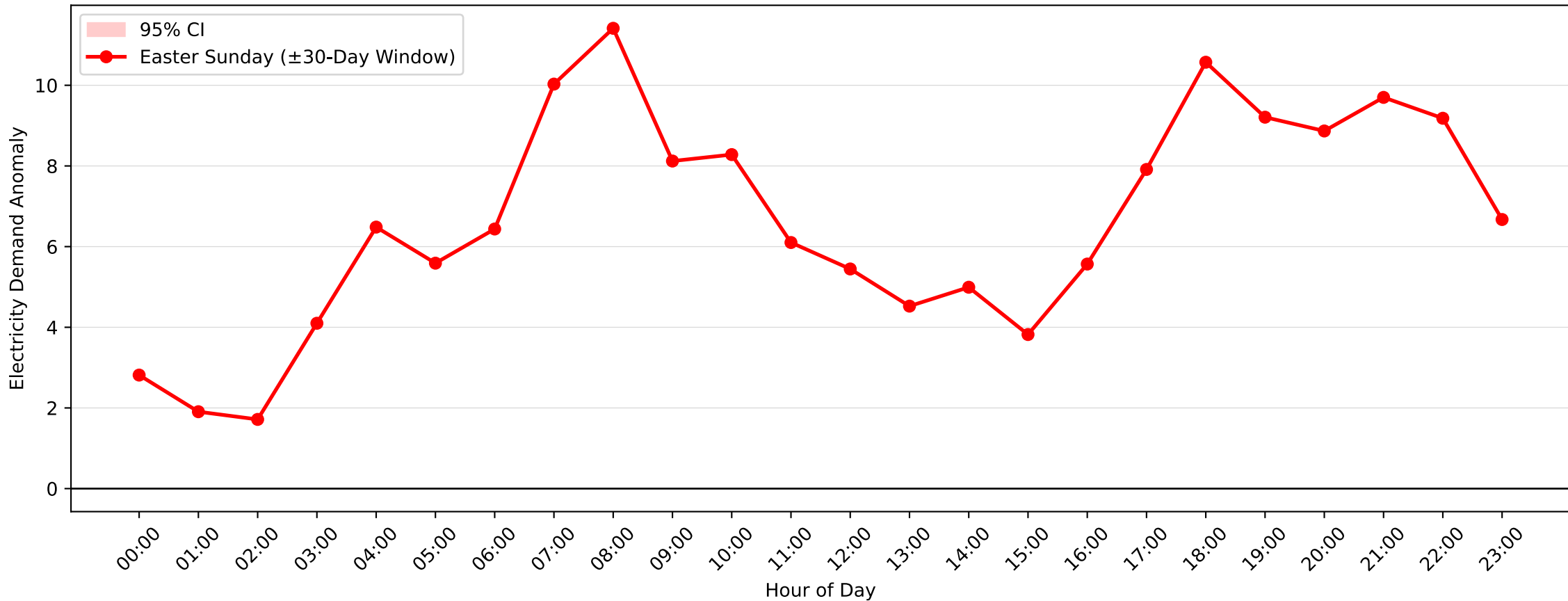
Greenacre Park Demand Anomaly: Easter Sunday (2004–2005, \pm 30 -Day Window)
