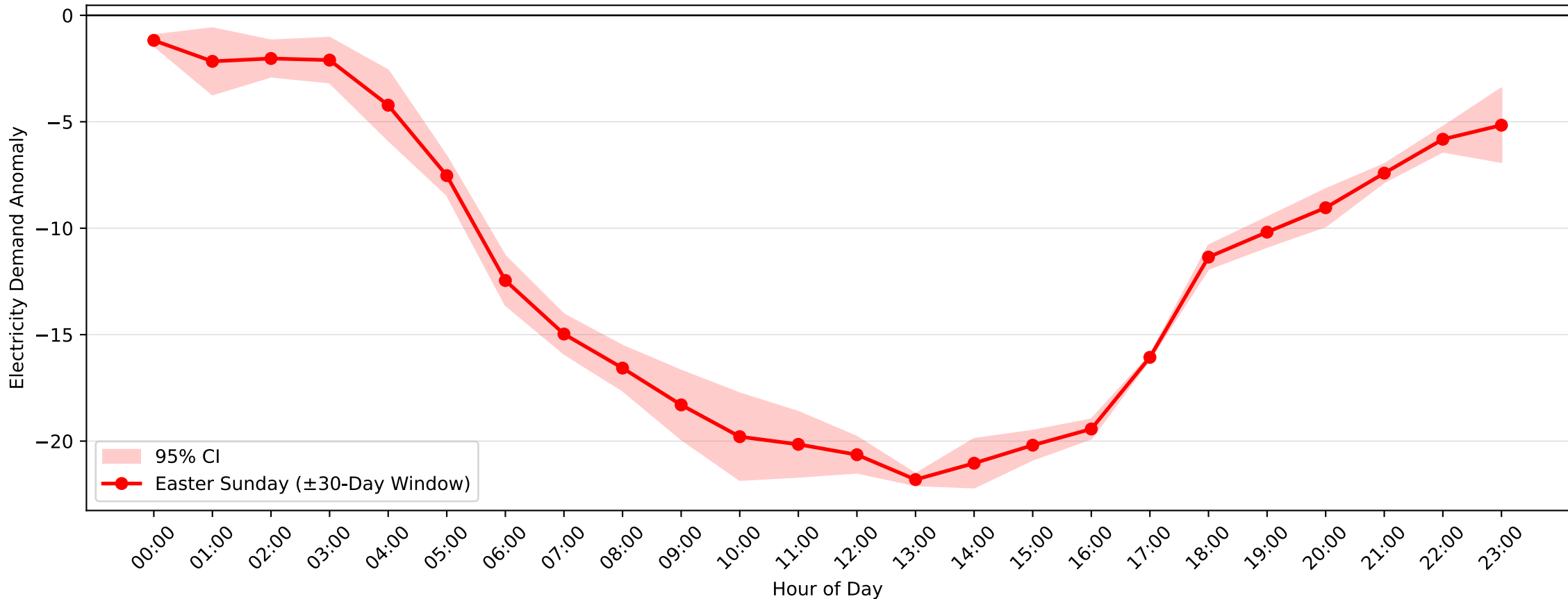
Greenacre Park Demand Anomaly: Easter Sunday (2006–2007, \pm 30 -Day Window)
