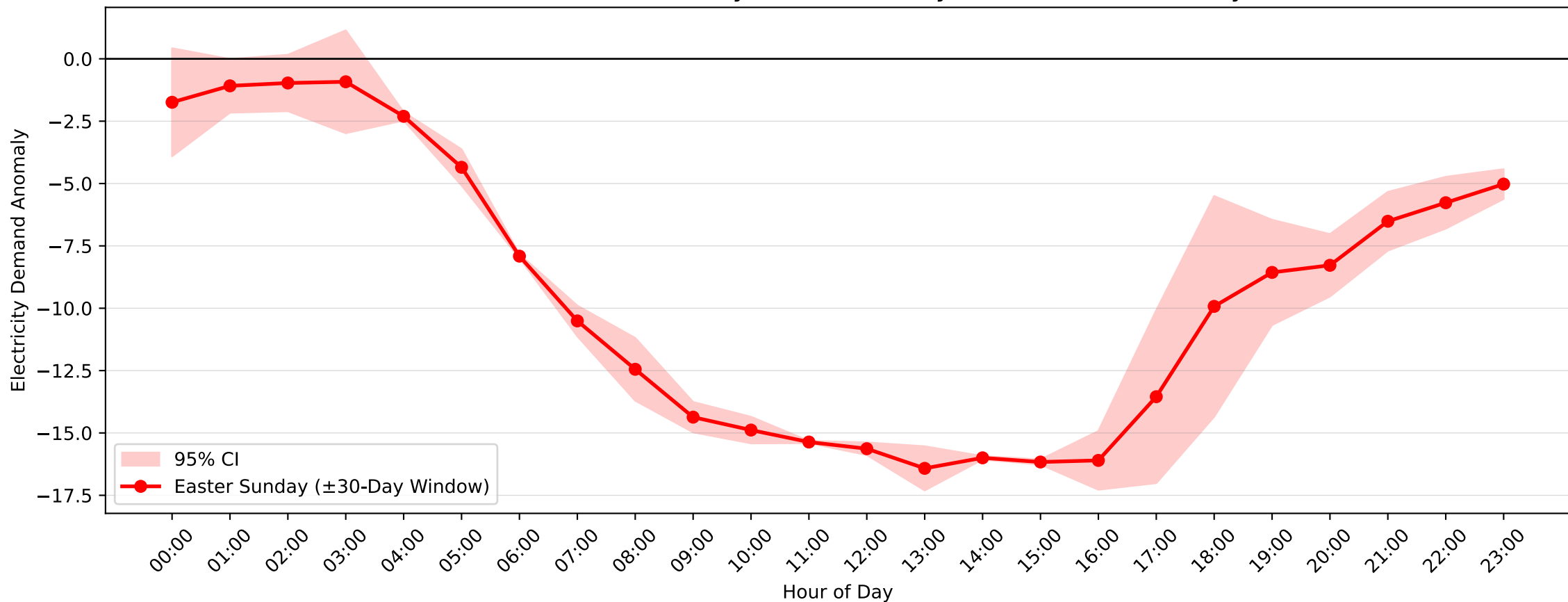
Greenacre Park Demand Anomaly: Easter Sunday (2012-2013, \pm 30 -Day Window)
