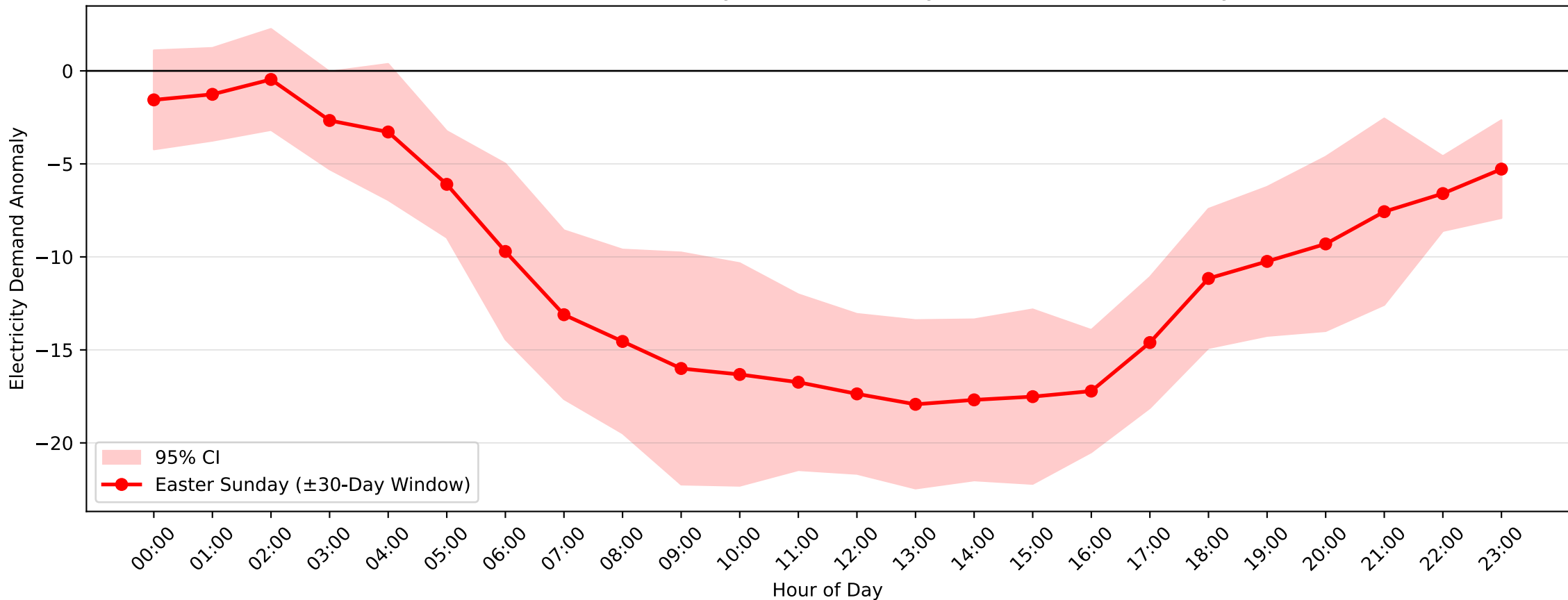
Greenacre Park Demand Anomaly: Easter Sunday (2010-2011, \pm 30 -Day Window)
