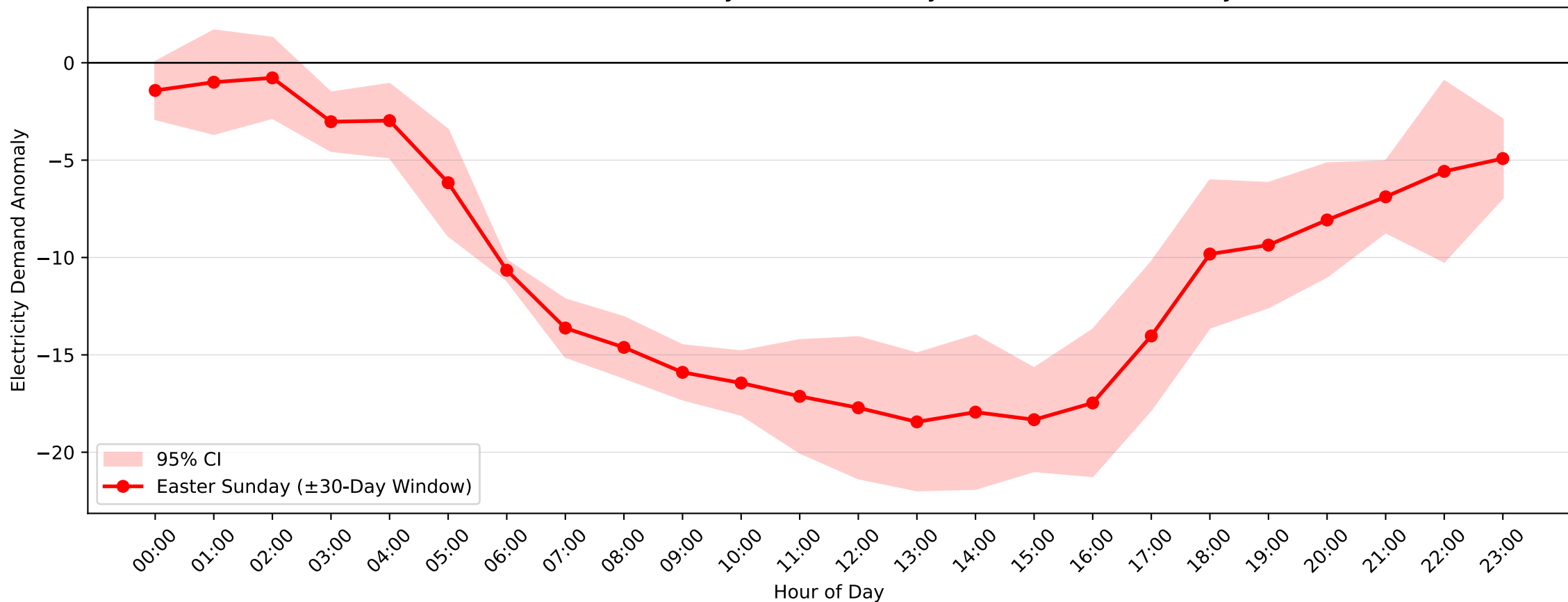
Greenacre Park Demand Anomaly: Easter Sunday (2009–2010, \pm 30 -Day Window)
