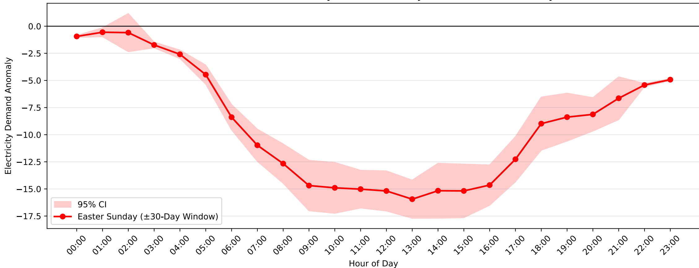
Greenacre Park Demand Anomaly: Easter Sunday (2011-2012, \pm 30 -Day Window)
